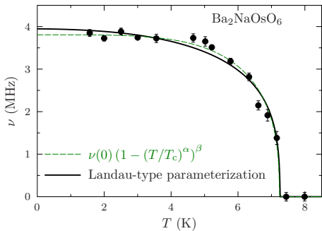
Figure 3: The frequency \nu(T) extracted from fits to A(t) spectra as a function of sample temperature T , along with fits to various models (see text). Data are only shown for the larger frequency \nu_1 because \nu_2 was held in fixed proportion during fitting (see text).
