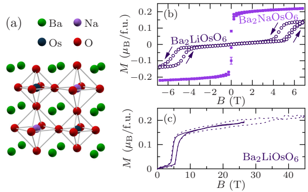
Figure 1: (a) Double-perovskite crystal structure. Alternation of \text{OsO}_6 octahedra (top left and bottom right) and \text{NaO}_6 octahedra, with barium ions occupying the remaining space. (b) Magnetization measured at 2 K in a SQUID magnetometer for \text{Ba}_2\text{MOsO}_6 . (c) Magnetization measured at 4 K in pulsed field for \text{Ba}_2\text{LiOsO}_6 , calibrated against the SQUID magnetization data. Data from a 45 T shot (dashed line) are noisier than those from a 25 T shot (solid line) but show no evidence for additional magnetic transitions.
